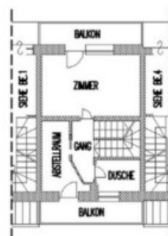
1.STOCK RH.2,60m
